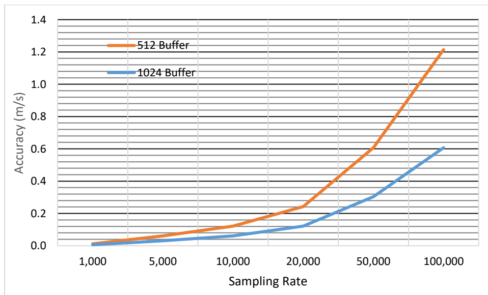
Figure 5. Buffer Size versus Accuracy
